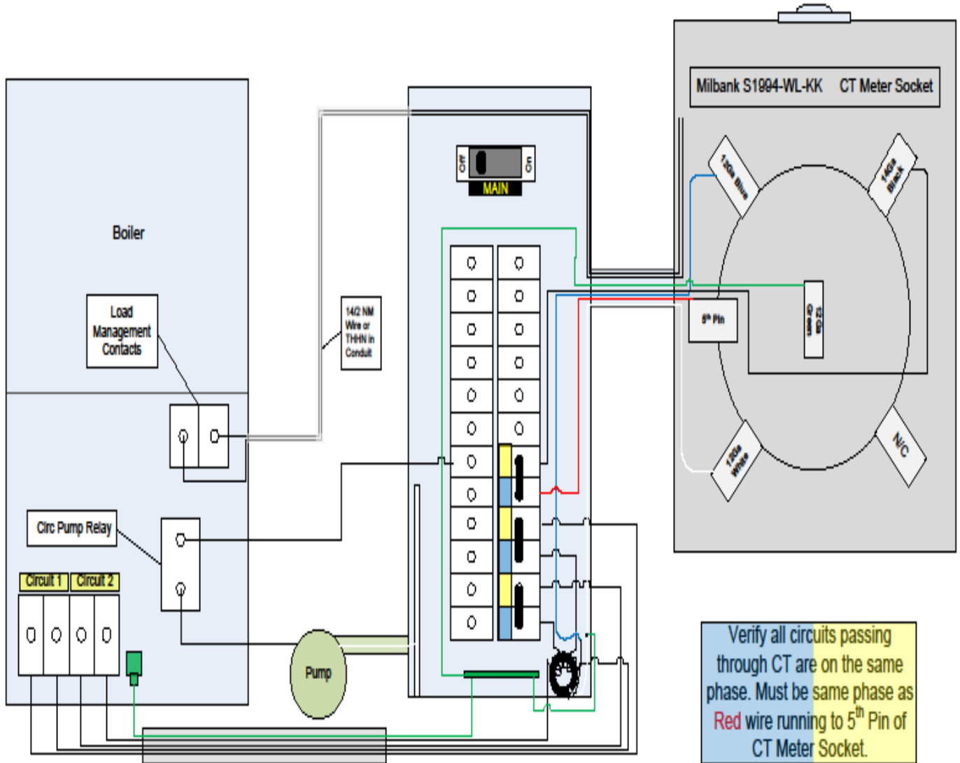
Typical Boiler Installation w/ CT Meter Socket
